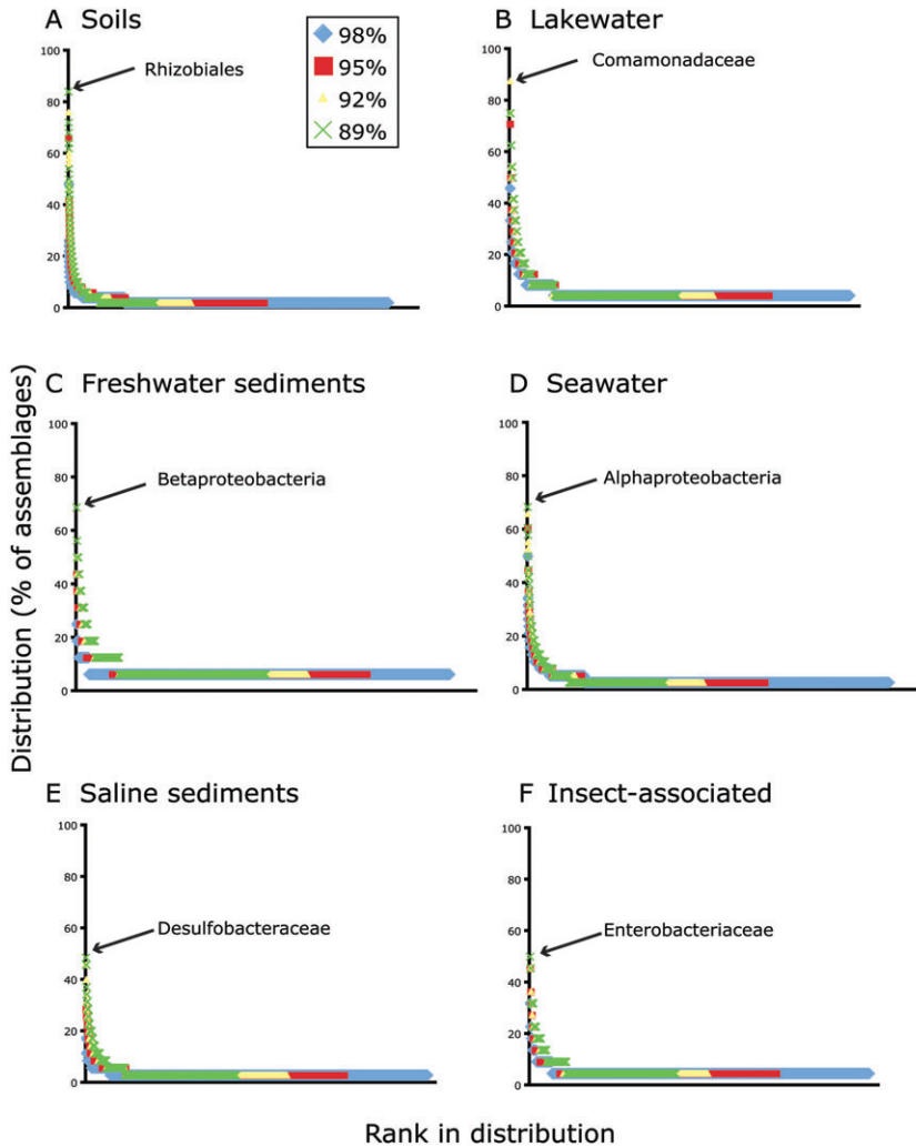
Fig. 3. The rank in distribution plotted against the per cent of assemblages each OTU was found in for (A) soils ( n = 49 ), (B) lakewater ( n = 21 ), (C) freshwater sediments ( n = 15 ), (D) seawater ( n = 40 ), (E) saline sediments ( n = 36 ) and (F) insect-associated samples ( n = 15 ) for the clone library data. Those OTUs that were most widely dispersed within habitat types are indicated. Within habitat types, some OTUs were widely distributed among assemblages while the majority were limited to only a few assemblages.
